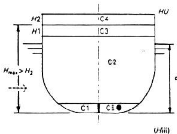
Figure A-10 - Interpretation of multiple horizontal subdivision (in all instances, r = 1 )
