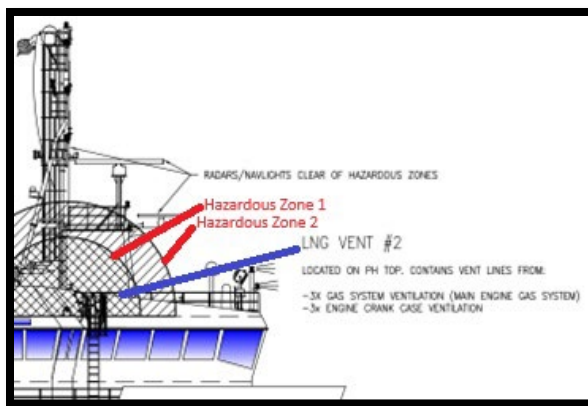
Figure 1 - Hazardous zone on air castle deck above pilothouse
